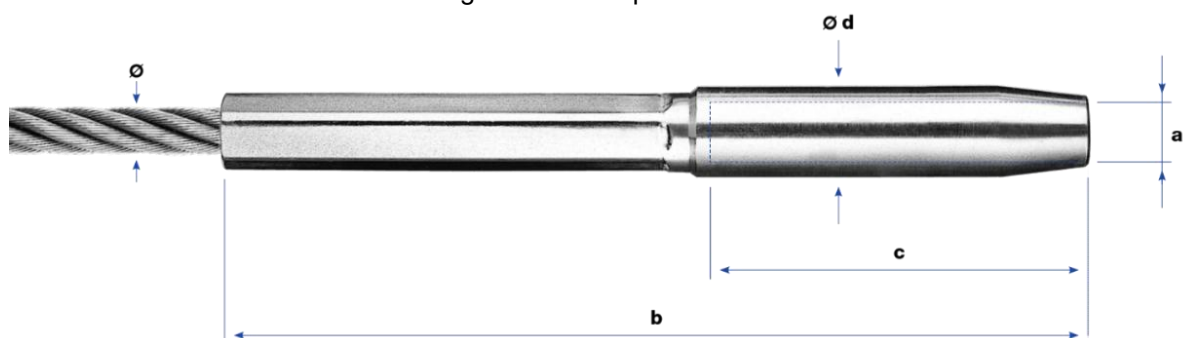
Figure above: rope Ø 10mm – 16mm
