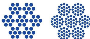
Applicable stranded rope constructions
