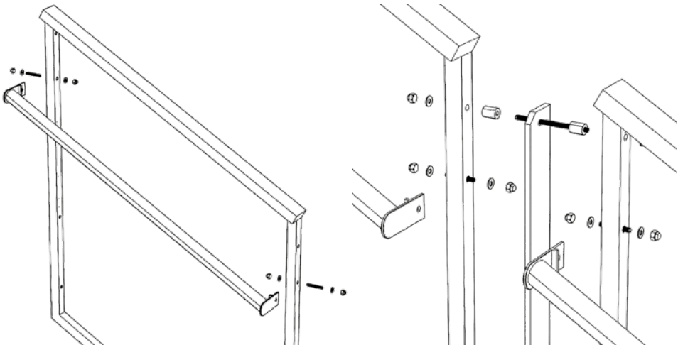
Installation drawing: Double handrail systems.
