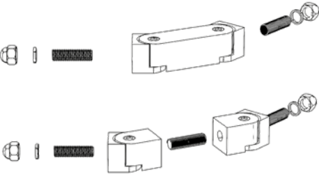
Installation drawing: Connectors enable smooth curved transitions.
