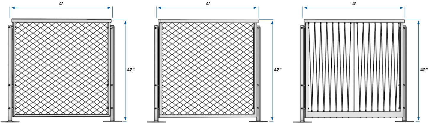
Frame round tube with Webnet
